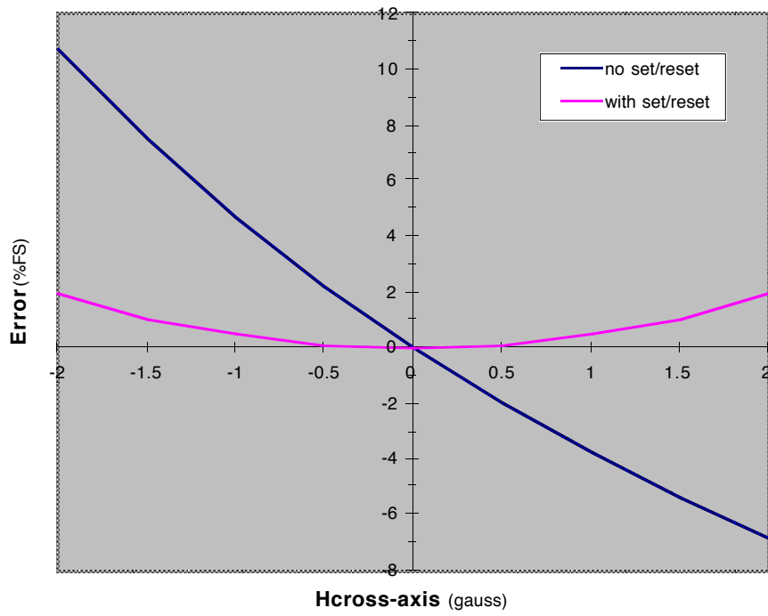
Cross-Axis Field Effect (Hsensitive=1.5 gauss)
