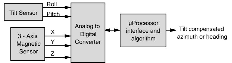
Figure 3—Compass system block diagram.
